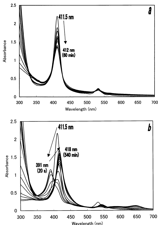
Figure 1. (a) The spectral changes under basic condition (aqueous acetonitrile solution (10% H 2 O) containing Ru II TMP(CO) (1.0 × 10 -5 M), K 2 Pt IV Cl 6 (5 × 10 -4 M), cyclohexene (1.0 × 10 -3 M), and KOH (1.5 × 10 -3 M)). (b) The spectral changes under neutral condition (aqueous acetonitrile solution (10% H 2 O) containing Ru II TMP(CO) (1.0 × 10 -5 M), K 2 Pt IV Cl 6 (5 × 10 -4 M), cyclohexene (1.0 × 10 -3 M), and KOH (0 M)).
